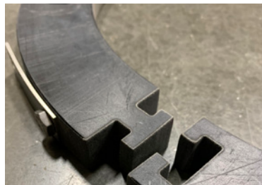
The Flush Ring is constructed of UHMWP with a notched seam for a more secure seal.
